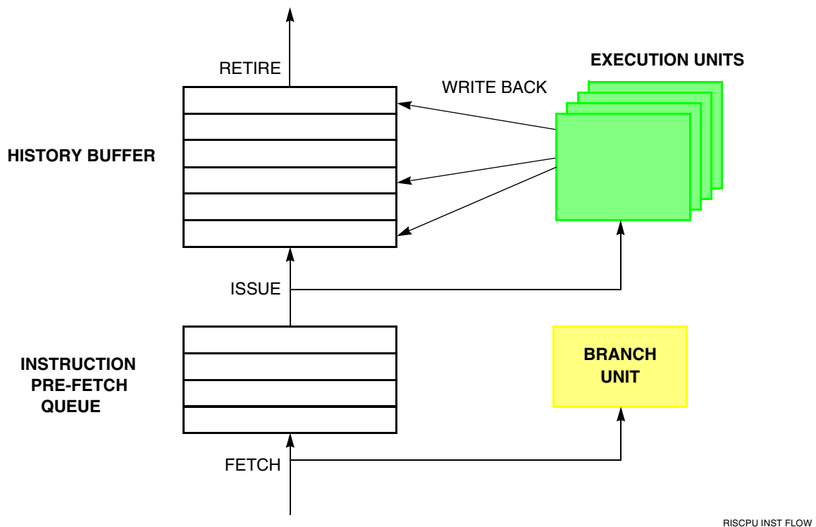
Figure 7-1 Instruction Flow
